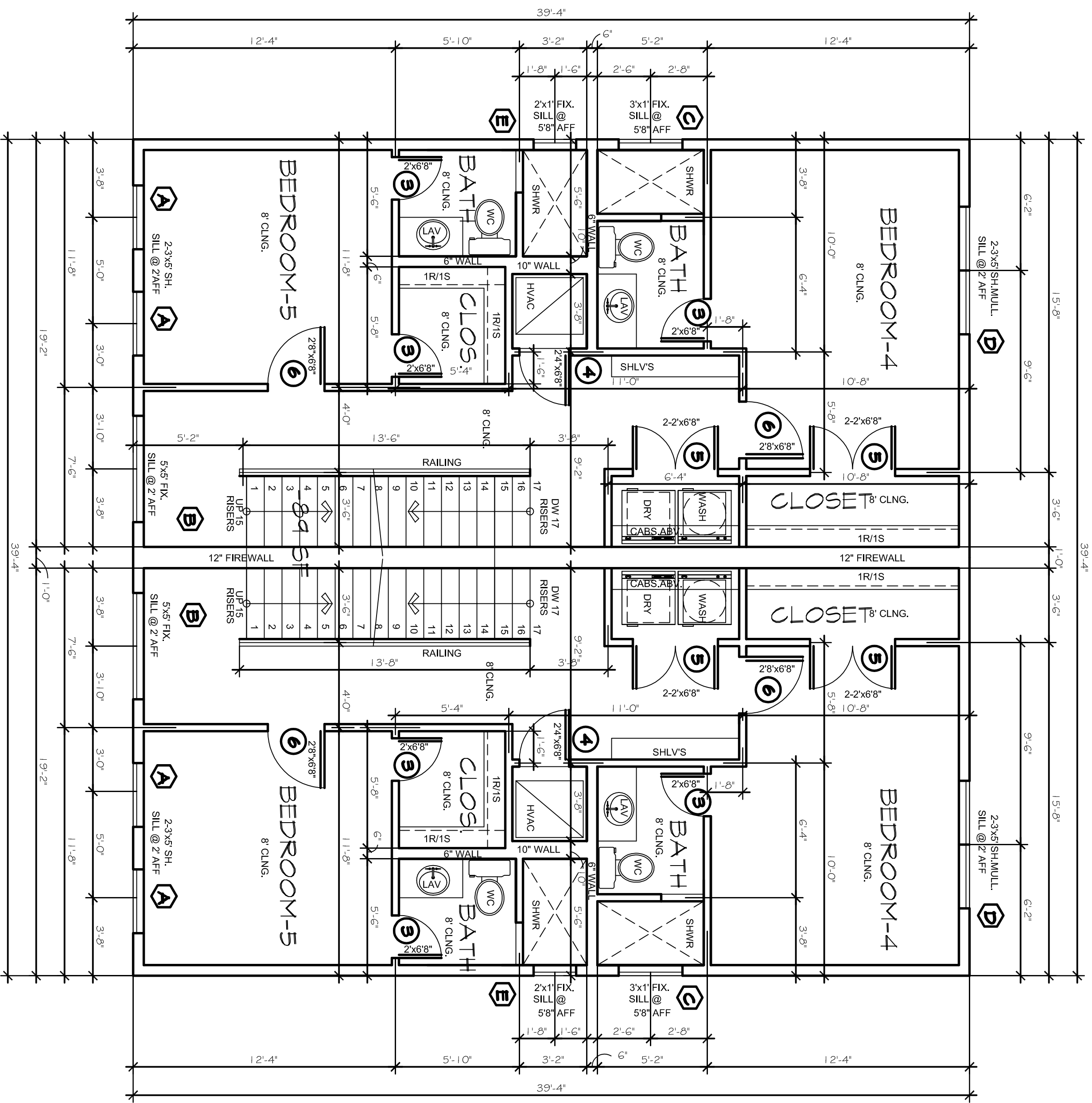
THIRD FLOOR SCALE: 1/4\"/>
