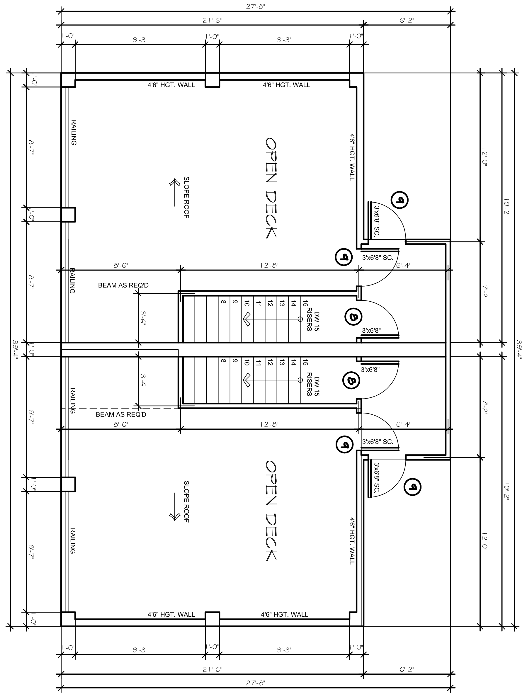
FOURTH FLOOR / ROOF PLAN SCALE: 1/16\"/>
