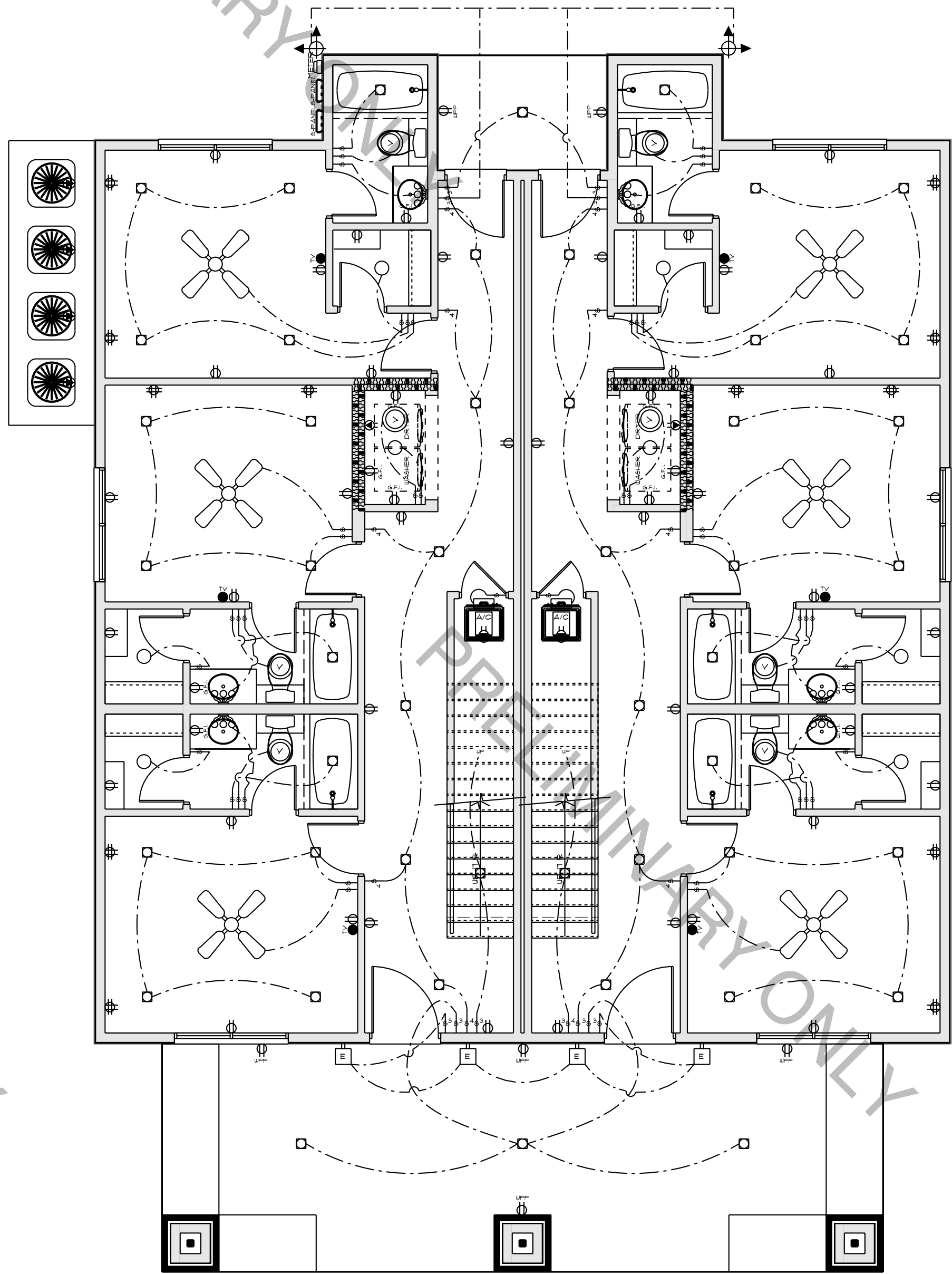
1ST FLOOR ELECTRIC PLAN
