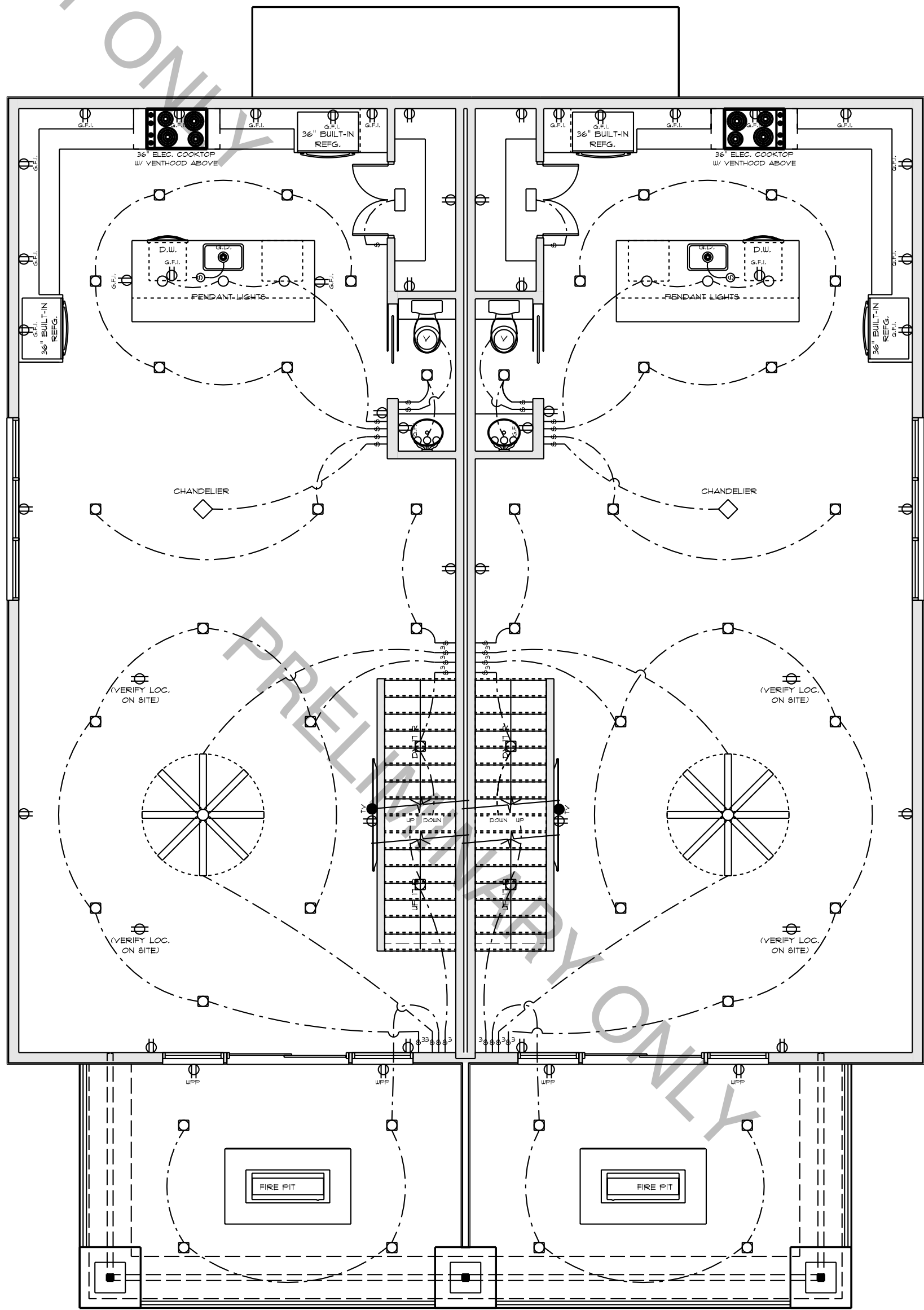
2ND FLOOR ELECTRIC PLAN
