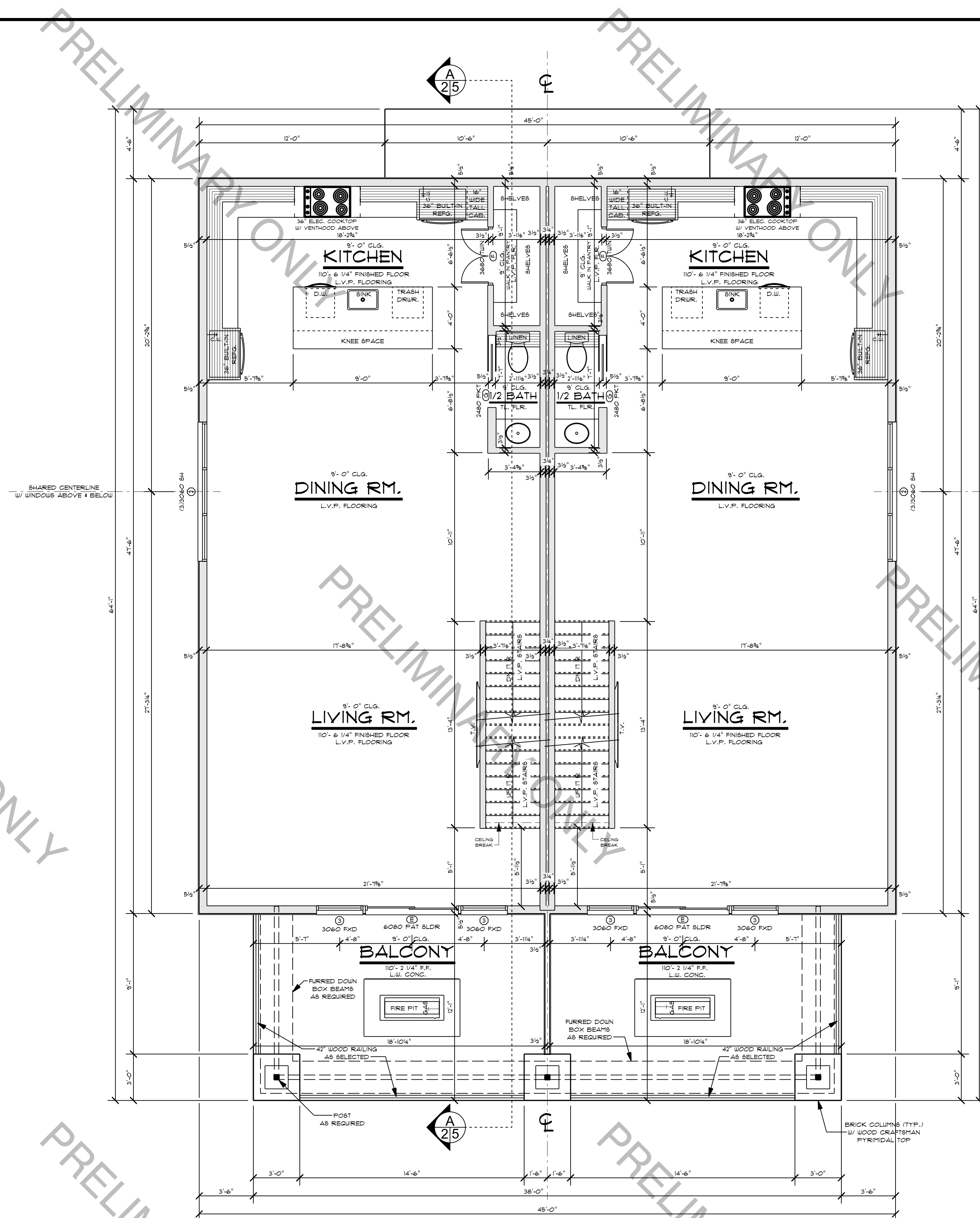
2ND FLOOR PLAN
