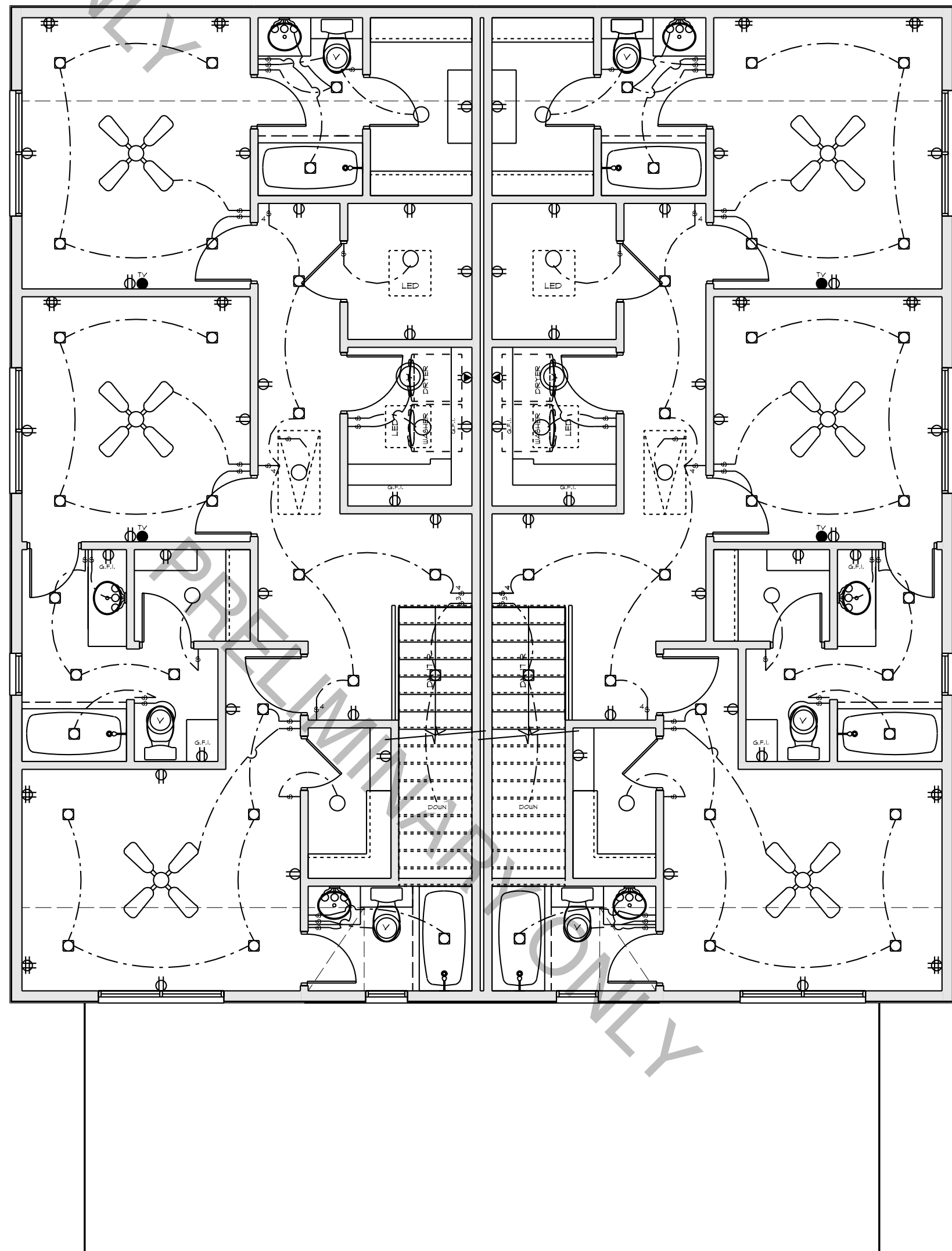
3RD FLOOR ELECTRIC PLAN
