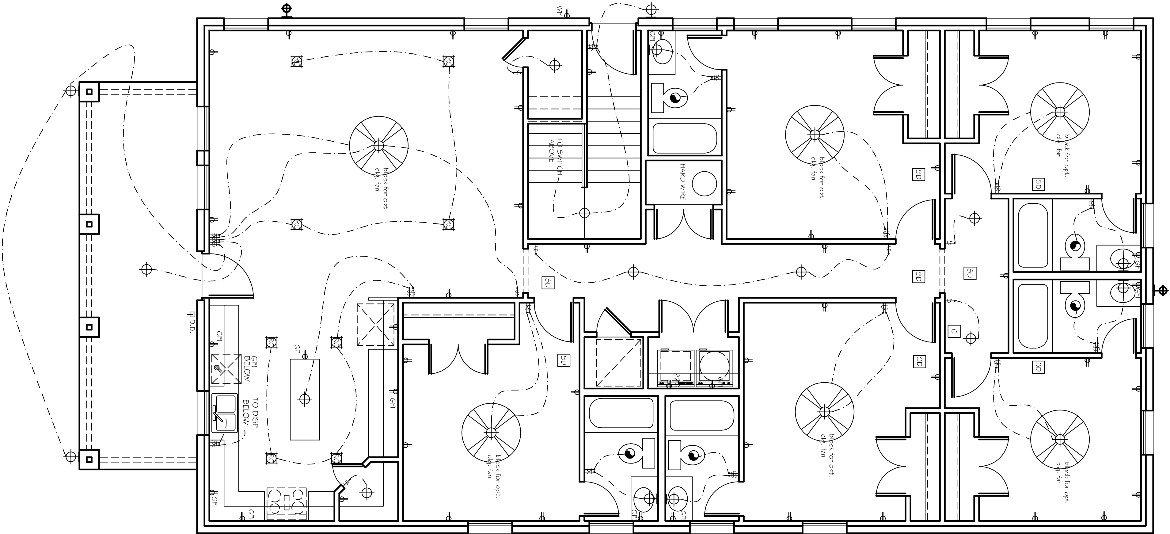
FIRST FLOOR ELECTRIC PLAN
