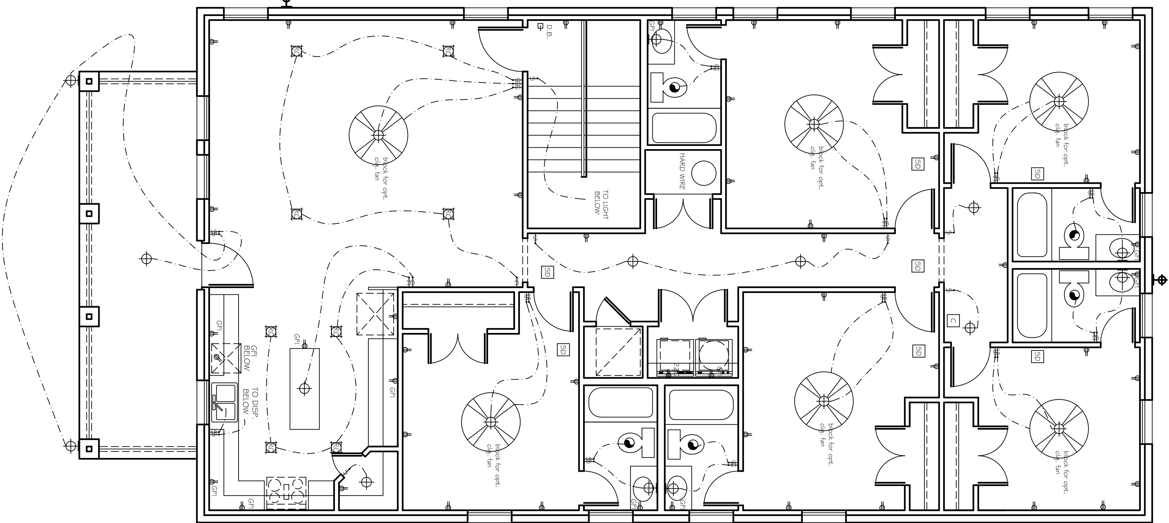
SECOND FLOOR ELECTRIC PLAN
