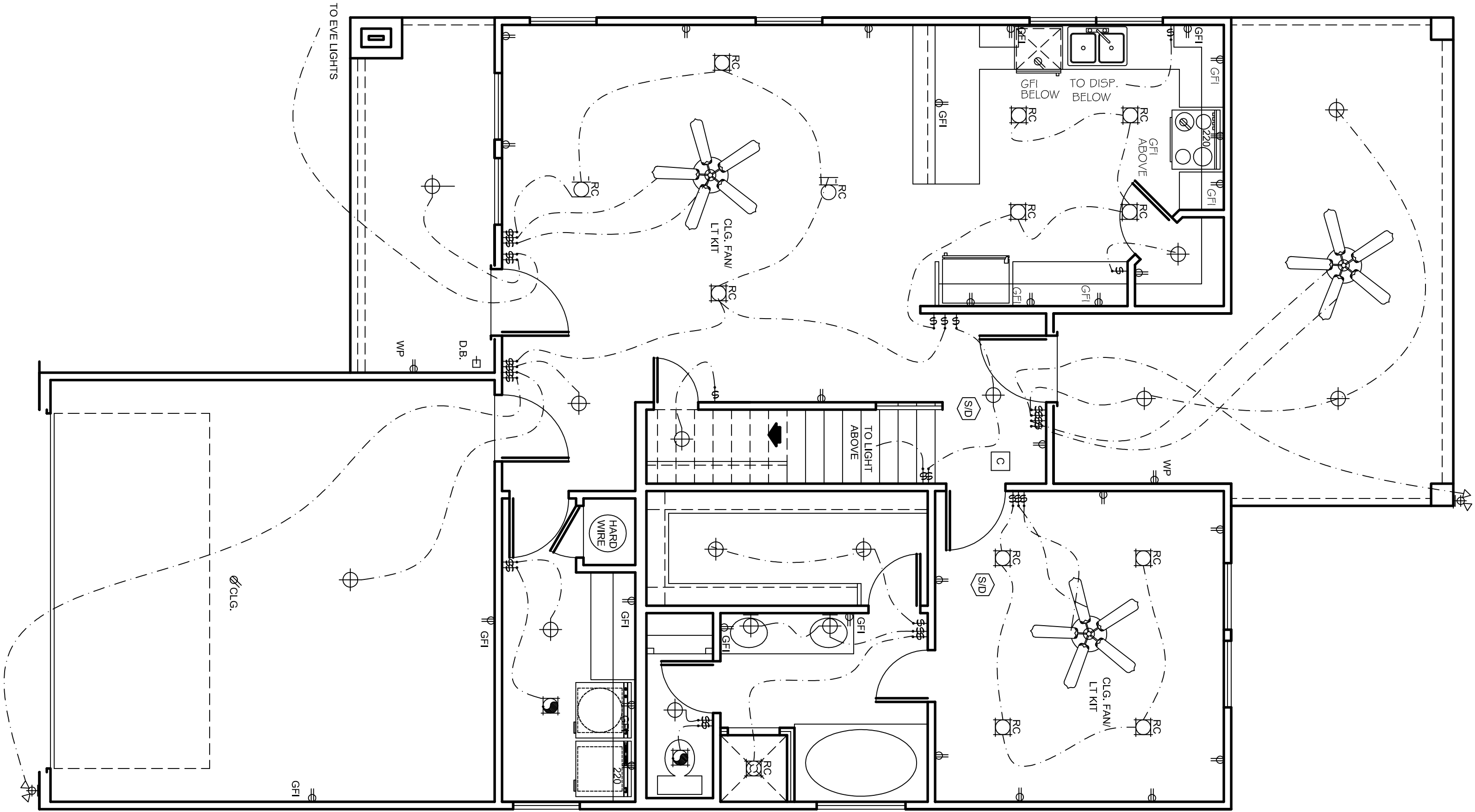
FIRST FLOOR ELECTRIC PLAN SCALE: 1/4"=1'-0"
