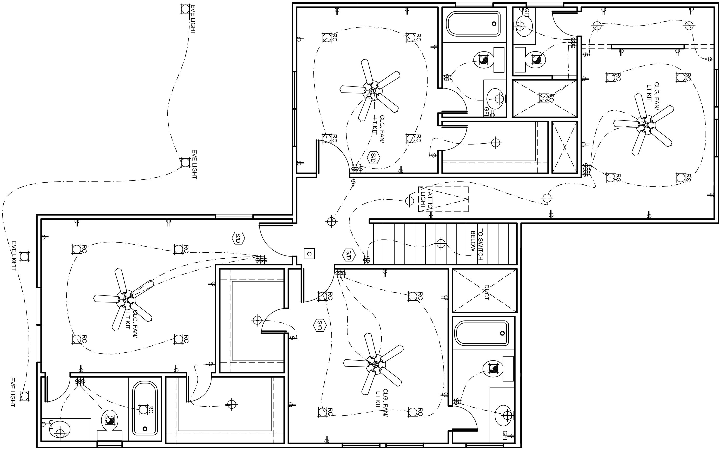
SECOND FLOOR ELECTRIC PLAN SCALE: 1/4"=1'-0"
