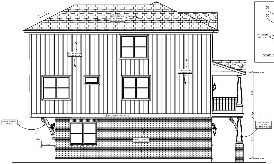
LEFT ELEVATION
