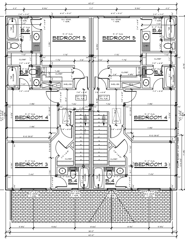
THIRD FLOOR PLAN SCALE: 1/4" = 1'-0"
